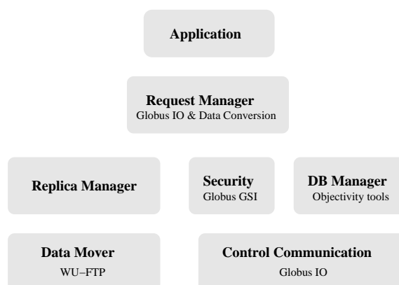
FIGURE 1. Logical datamodel of the tool
